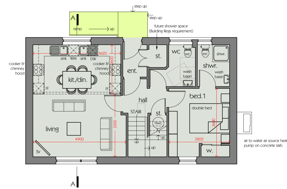
ground floor plan (gross internal floor area - 61m 2 approx.)
