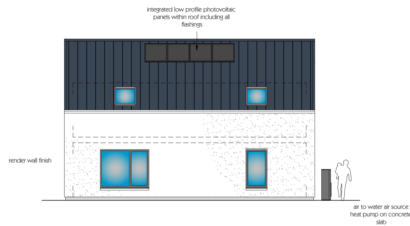
rear (south) elevation
