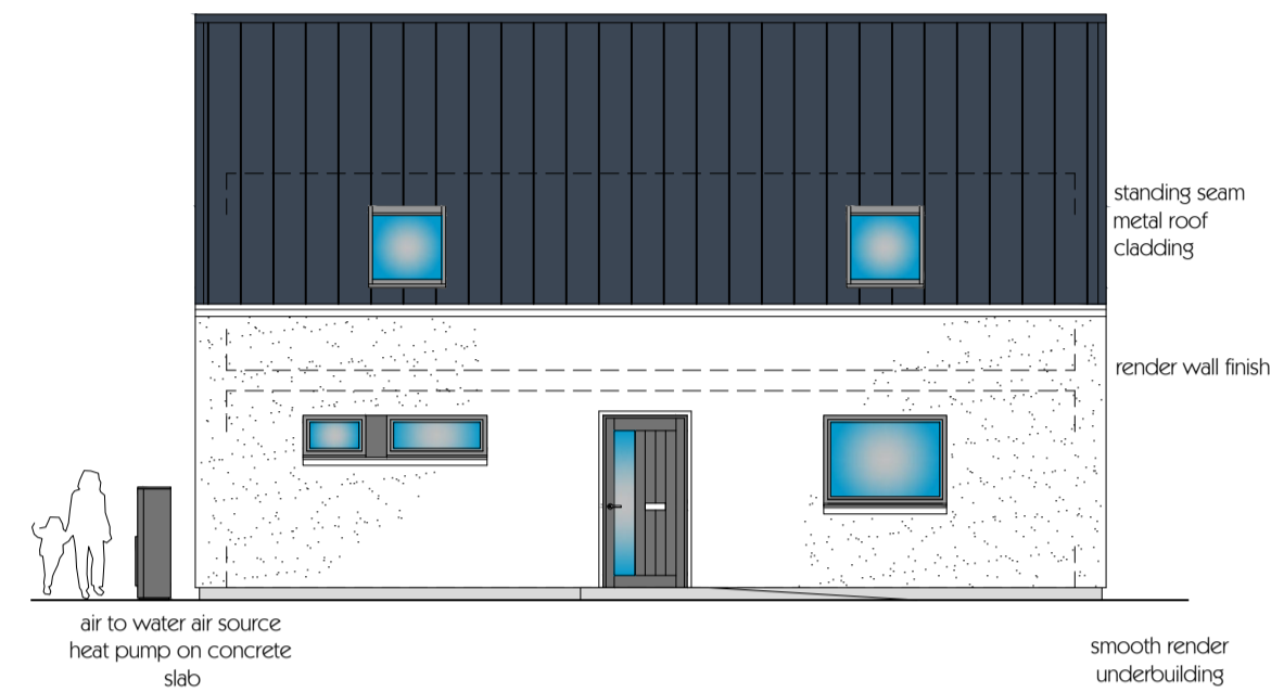
front (north) elevation
