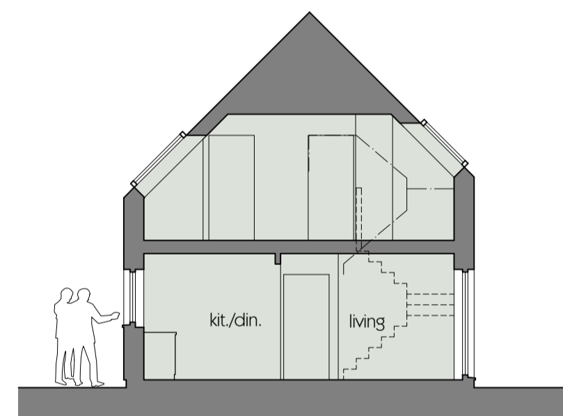
section AA
